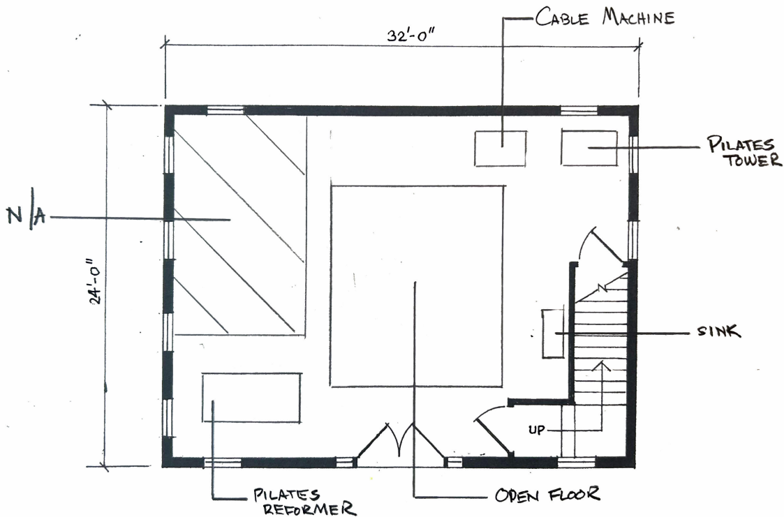
BUILDING 2 - FIRST FLOOR PLAN
