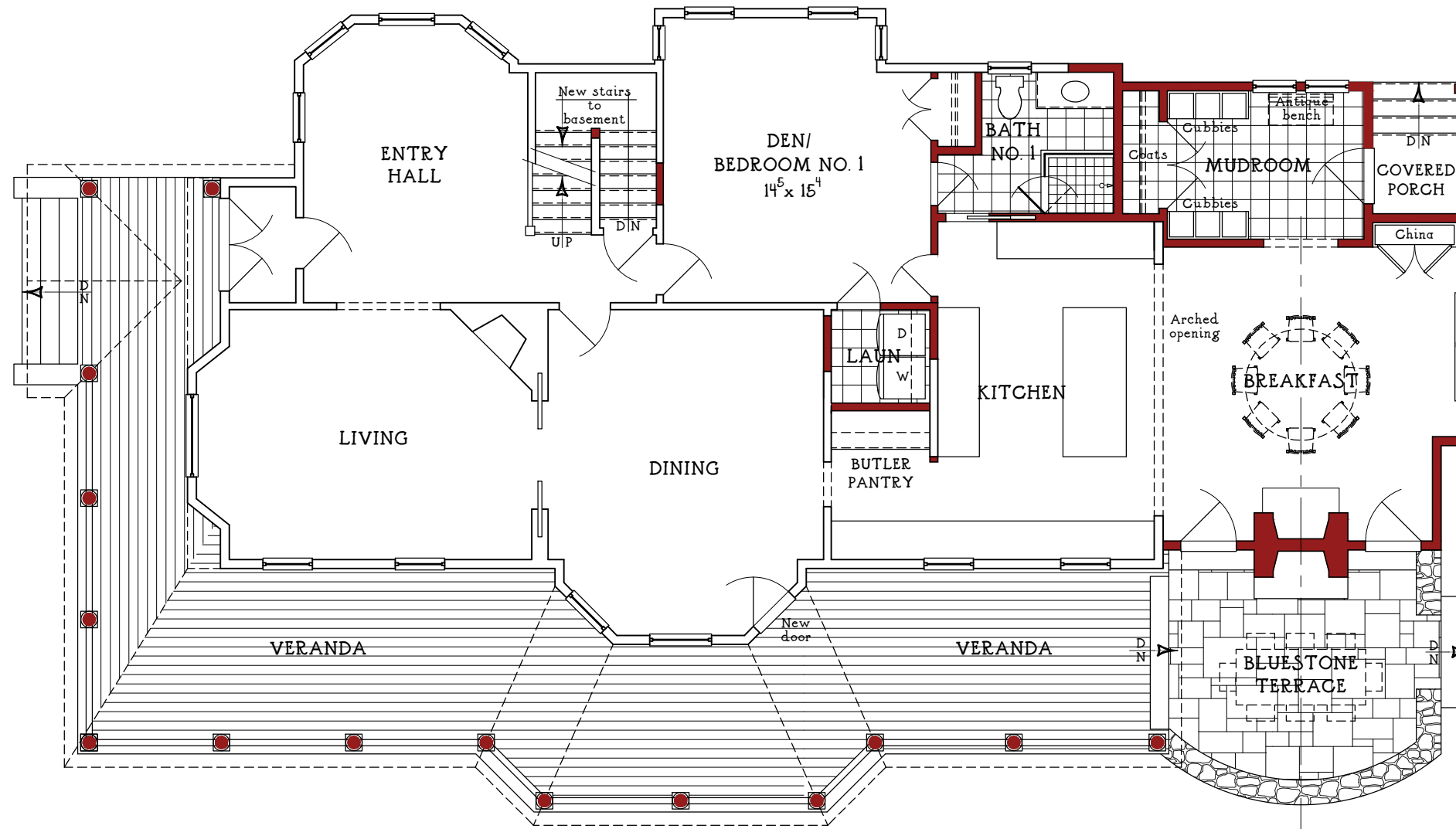
PROPOSED FIRST FLOOR PLAN - 1/8"
