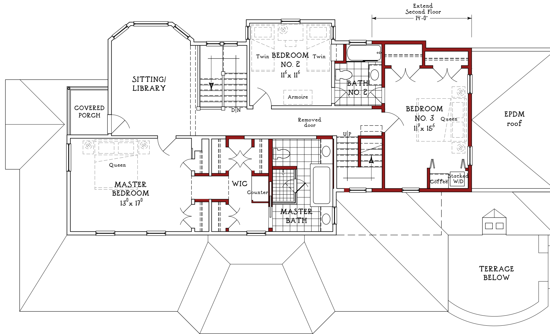
PROPOSED SECOND FLOOR PLAN - 1/8"
